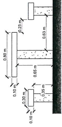
3 VISTA PRINCIPAL 1 : 25
